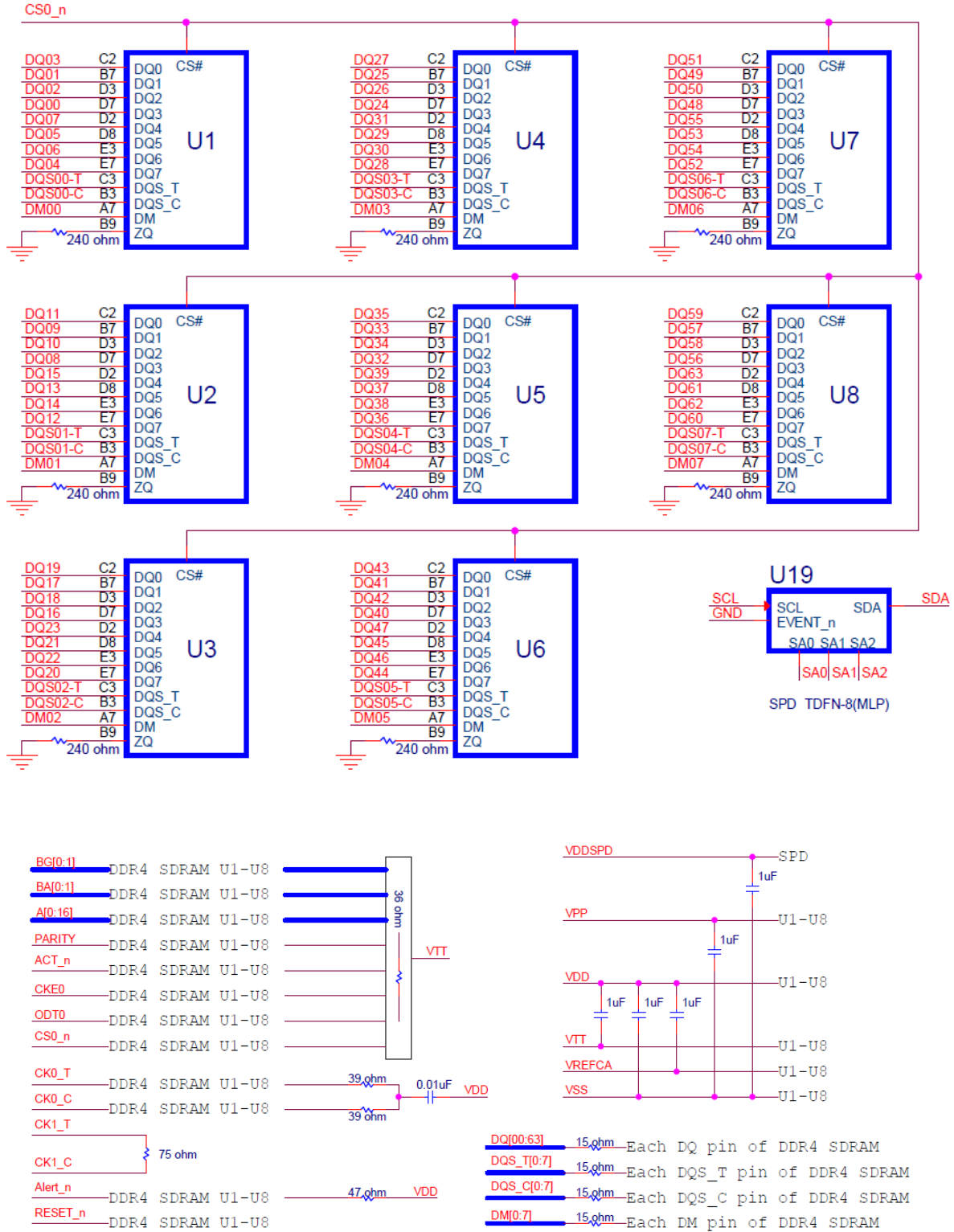
Figure 1 – Function Block Diagram_SCC08GU03H5F1C-32AA
