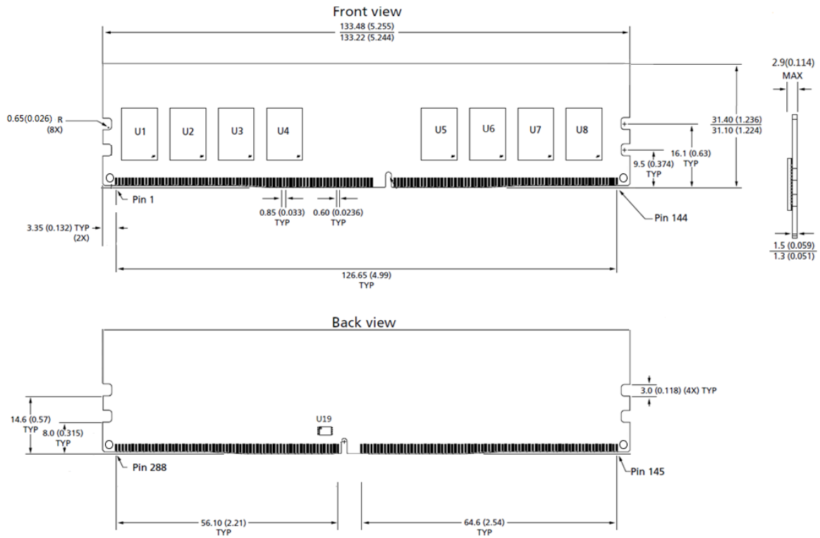
Figure 2 – Package Dimensions_SCC08GU03H5F1C-32AA
