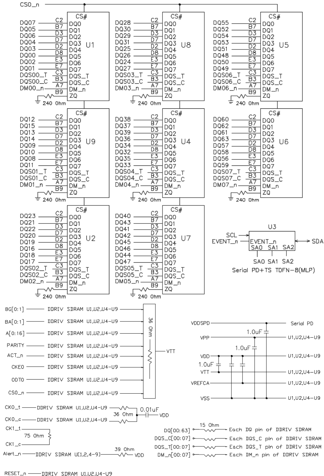
Figure 1 - Function Block Diagram_SCC08GS03H5F1C-32AA
