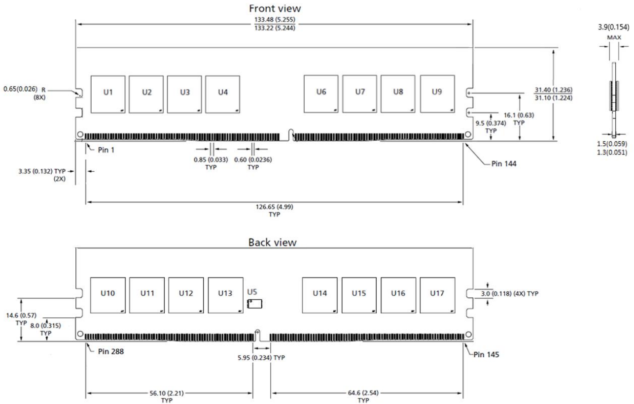
Figure 4 – Package Dimensions_SCC16GU13C2F1C-32AA
