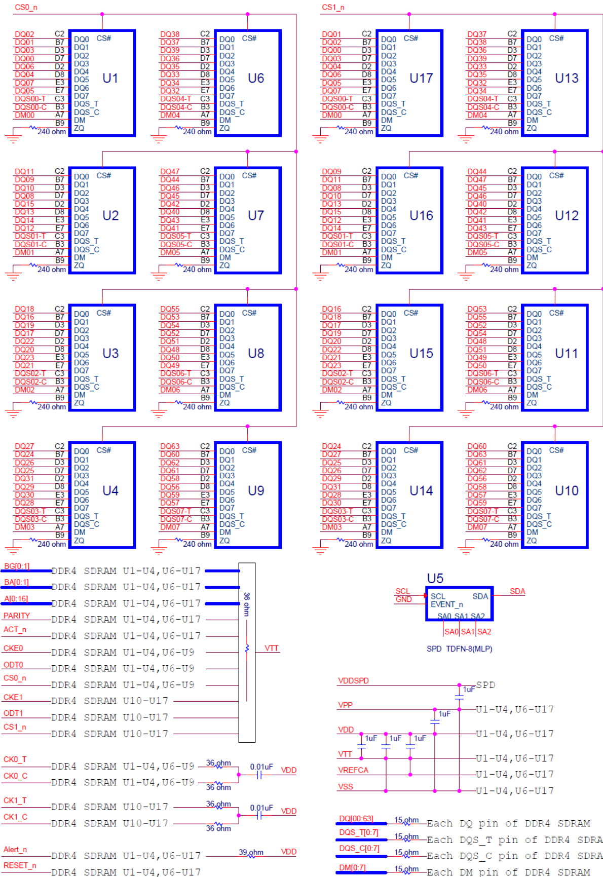
Figure 2 – Function Block Diagram_SCC16GU13C2F1C-32AA
