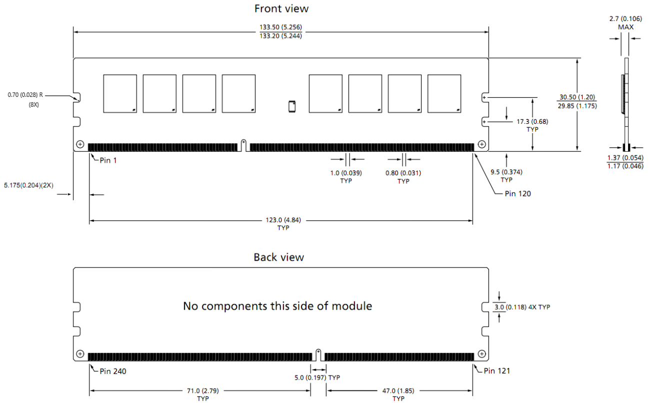
Figure 1 - Package Dimensions_ HXMSH4GU03A2F1C-16K
