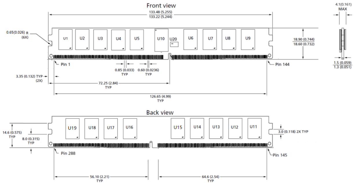
Figure 4 - Package Dimensions_SCC32GP13H4F1V-32AA
