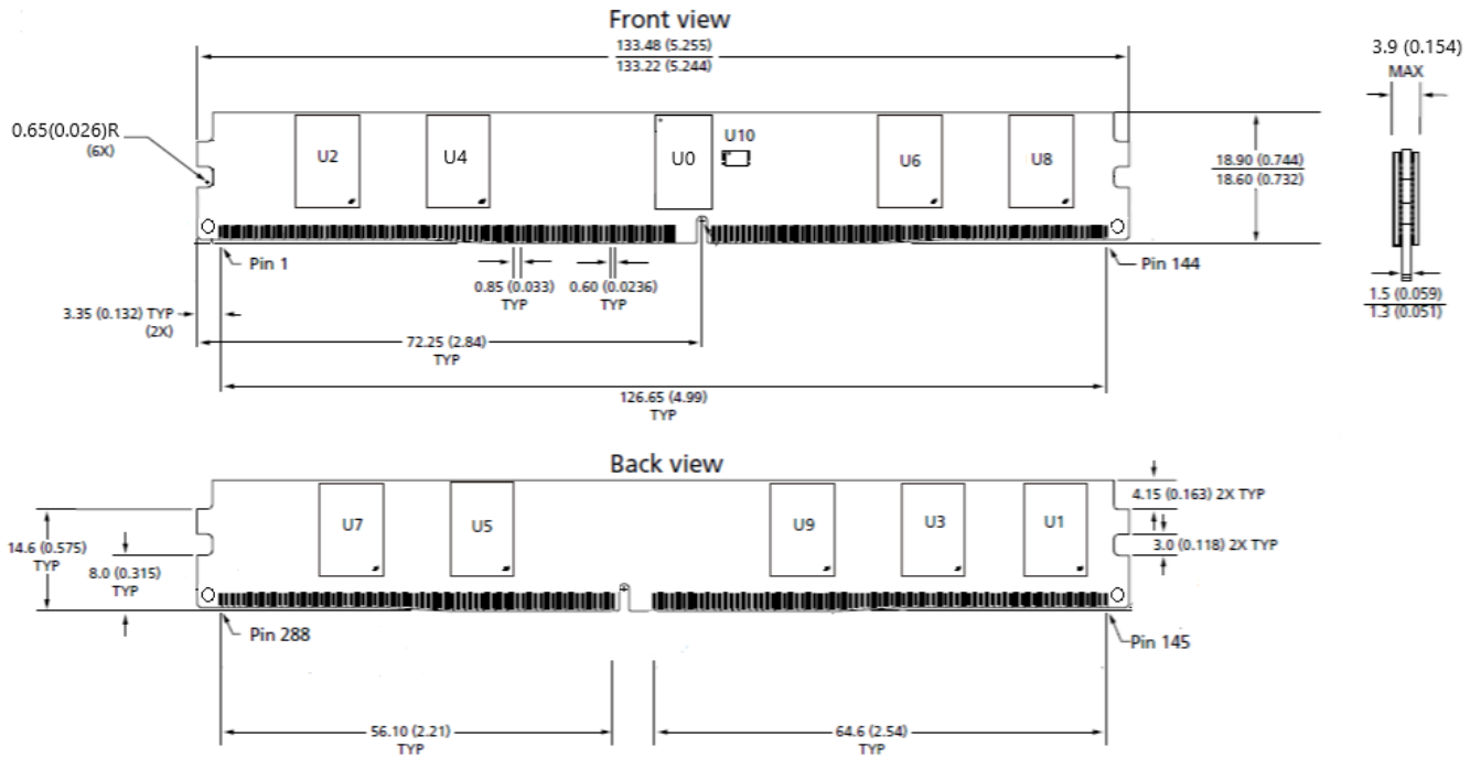
Figure 3 - Package Dimensions_SCC16GP03H4F1V-32AA
