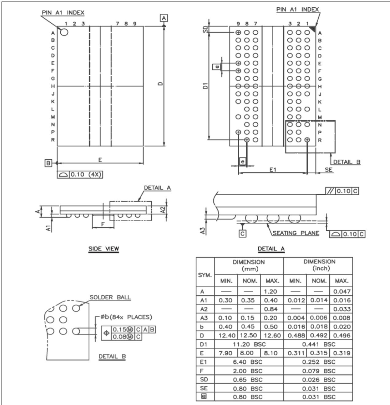
Figure 11 - Package Outline PG-TFBGA-84
