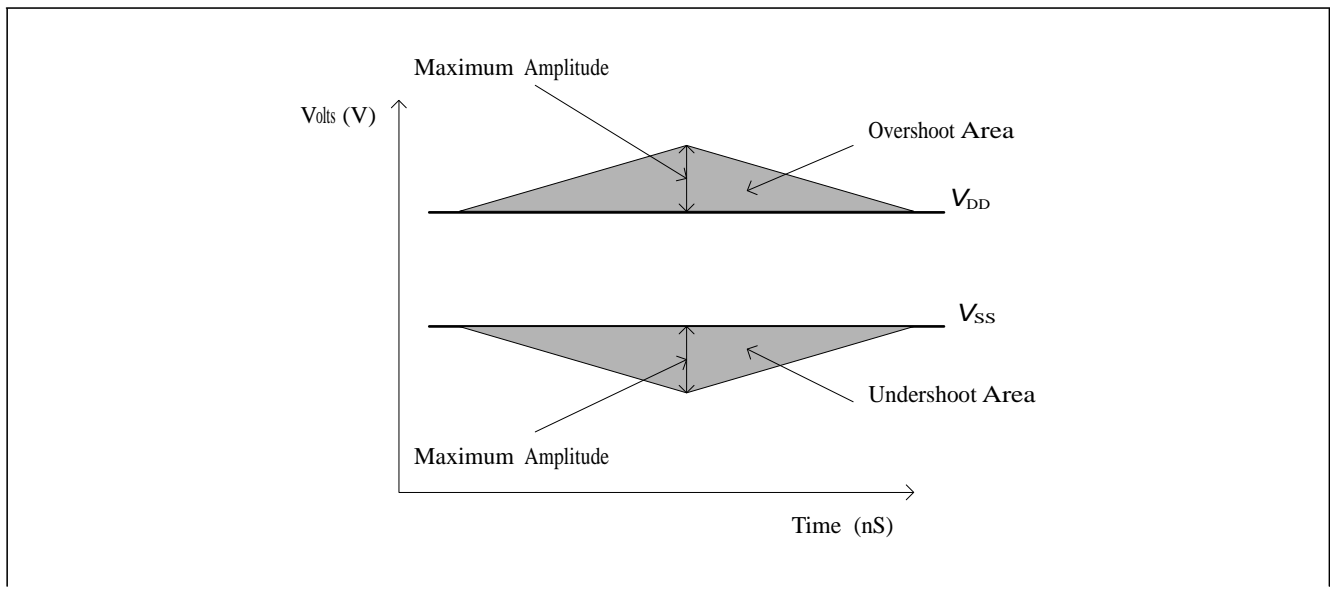
Figure 5 - AC Overshoot / Undershoot Diagram for Address and Control Pins
