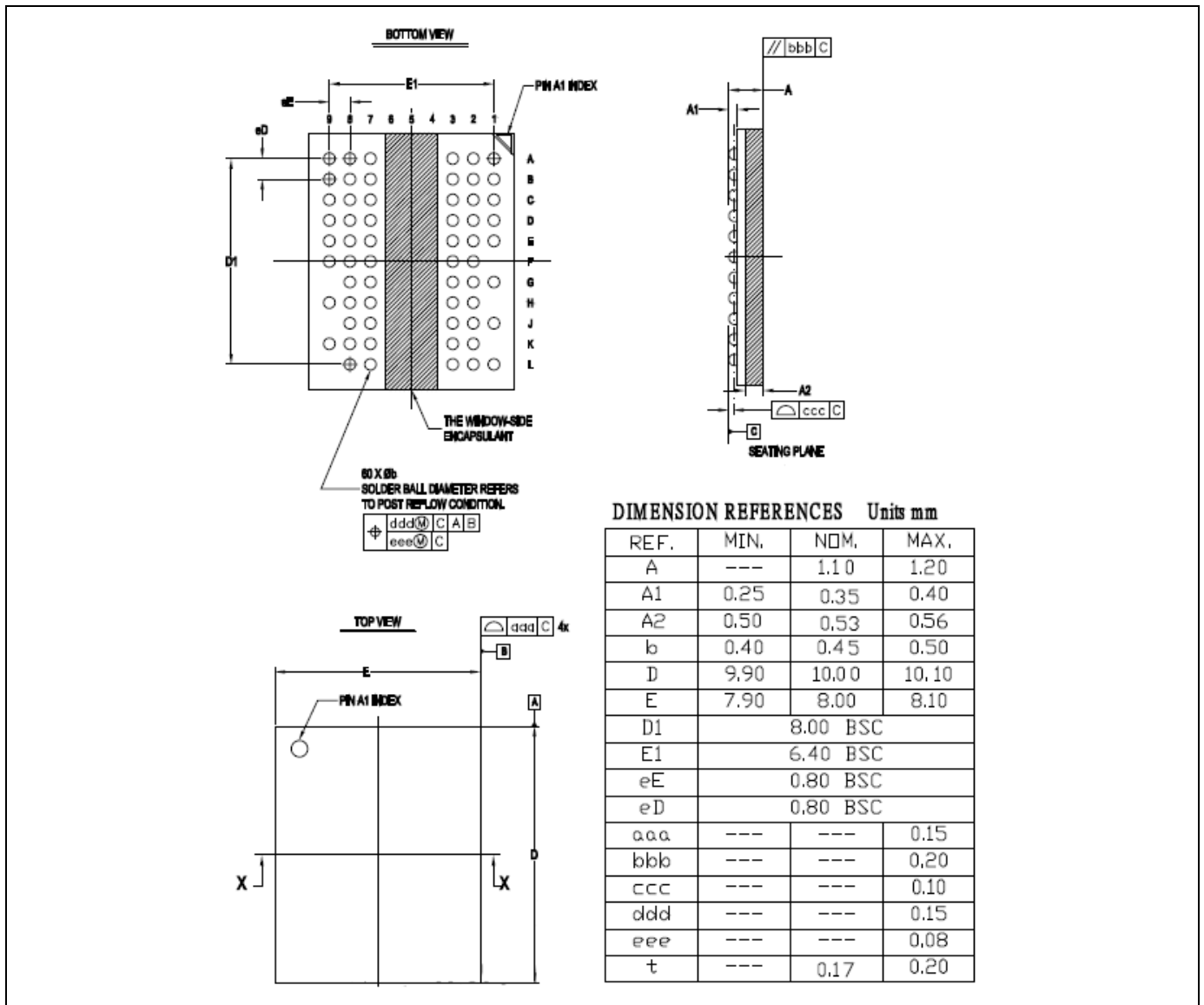
Figure 10 - Package Outline PG-TFBGA-60
